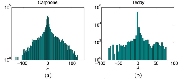
Fig. 1. (a) The log histogram of \mu_n for the natural image Carphone. (b) The log histogram of \mu_n for the depth map Teddy.
